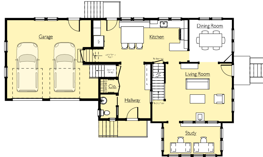
2 First Floor Plan - After
