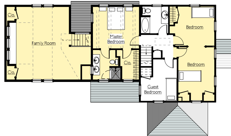
4 Second Floor Plan - After
