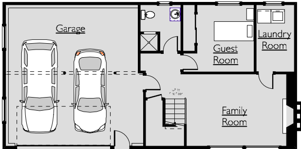
1 First Floor Plan - Before
